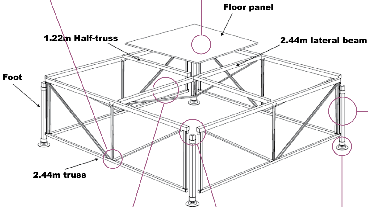
Truss - half-truss
